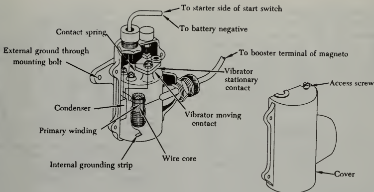
FIGURE 4-20. Booster coil.
